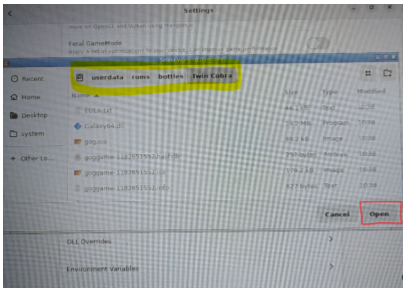
Working directory
